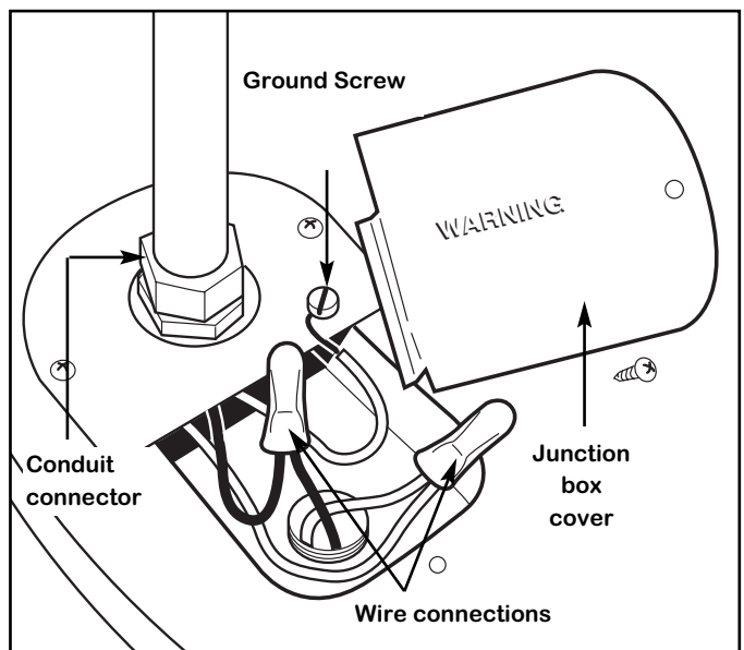
Figure 3. — Water Heater Junction Box showing typical wiring method and connections.
