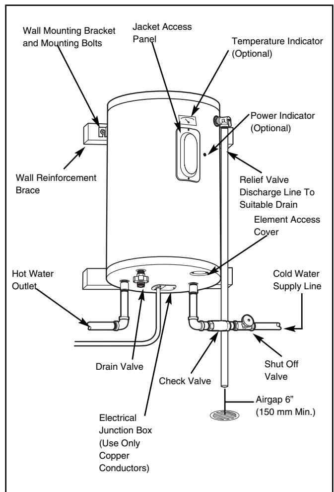
Figure 2. — Typical Vertical Installation
